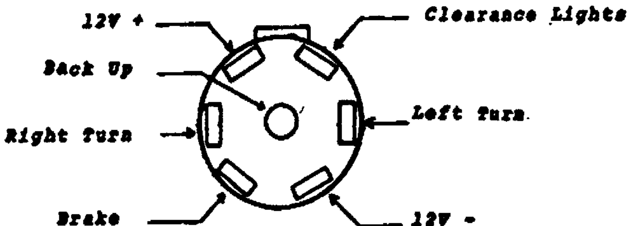
7-WAY PLUG - TRAILER END
